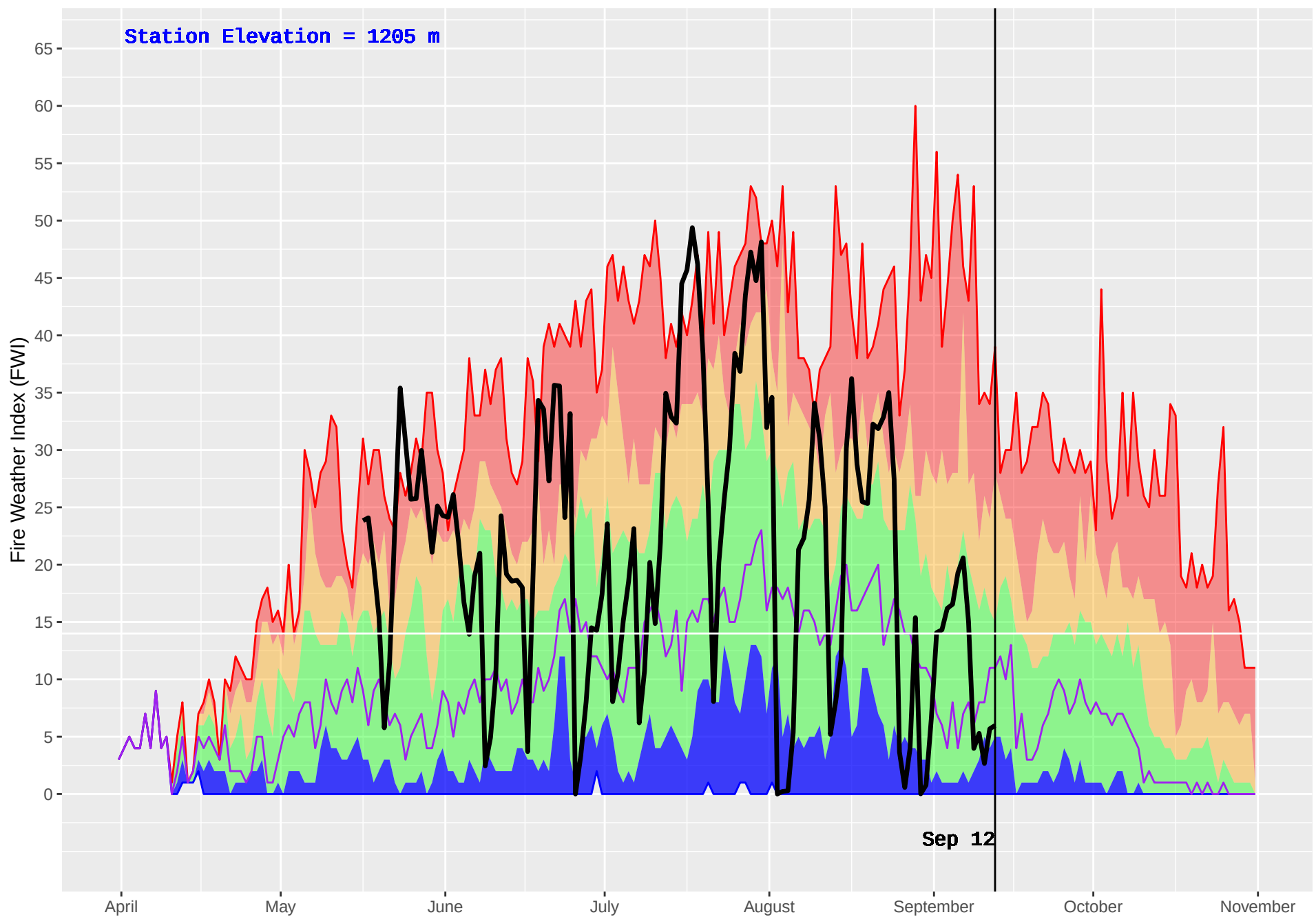
GWYNETH LAKE (309) : Historical (1986–2016) and Current (2018) Daily Fire Weather Index (FWI)
